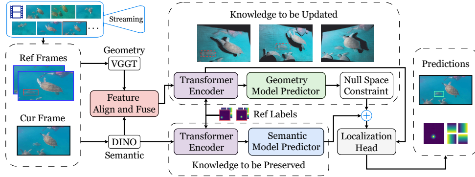
Figure 1: The GOT-Edit Framework. GOT-Edit facilitates the understanding of 3D geometry to aid generic object tracking from 2D streaming inputs. It predicts semantic and geometric model weights concurrently to incrementally adapt the tracking model. Through online model editing, it ensures geometry-aware, semantic-preserving updates to the tracking model. The solid red box marks the ground-truth target in the input reference frames. The dashed red boxes indicate these same annotations utilized for the online knowledge update within the geometry branch. The green box represents the final predicted tracking result.
