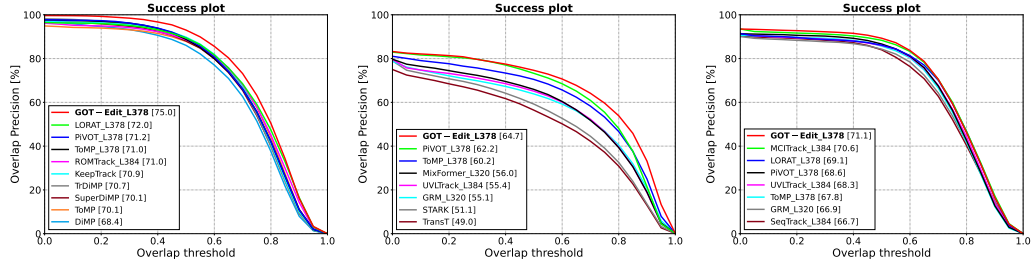
Figure 2: From left to right, success plots of competing methods on OTB, AVisT, and NfS are shown.
