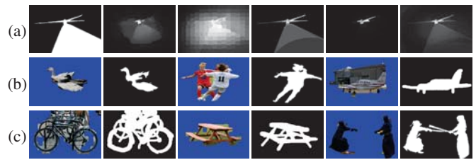
Fig. 13: Some challenging cases/examples where our method fails. (a) Most of the saliency proposals do not perform well. From left to right, the ground truth, four adopted SISMs from DSR, MR, DRFI and RBD, and our fused map are shown. (b) Multiple similar objects are present and/or the goal is to extract a particular object instance. (c) Objects of interest have complex shapes or long-thin boundaries.
