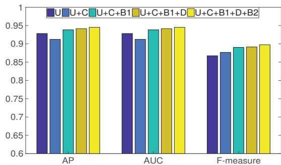
Fig. 10: Ablation studies on the Image-Pair dataset in AP, AUC, and F-measure ( F_\beta ).
