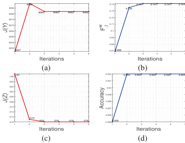
Fig. 12: Learning curves during optimizing (3) on the Image Pair dataset. (a) The objective values of (17). (b) The weighted F-measure scores of co-saliency detection. (c) The objective values of (18). (d) The accuracy scores ( \mathcal{A} ) of co-segmentation.
