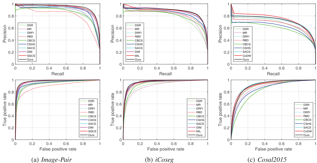
Fig. 6: Performance of co-saliency detection in PR and ROC curves on three benchmark datasets including the (a) Image-Pair, (b) iCoseg, and (c) Cosal2015 datasets. The models adopted to generate our fusion proposals are plotted in dash lines, while the state-of-the-art co-saliency detection methods are in solid lines.
