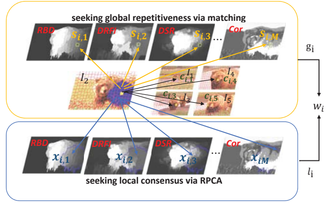
Fig. 4: Illustration of the unary term U term for co-saliency detection. See the text for the details.
