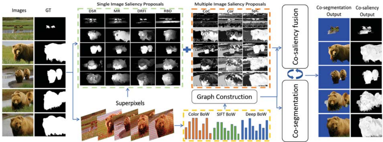
Fig. 3: The proposed framework for joint co-saliency detection and co-segmentation. Given images of a particular object category, we process the input images by compiling their superpixel representation, extracting features from the superpixels, and computing a set of saliency proposals. The proposed approach takes the processed data as input, and performs alternating co-saliency detection and co-segmentation until convergence.
