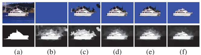
Fig. 11: Visual illustration of ablation studies. (a) An image from the Image-Pair dataset and its ground truth for joint co-saliency detection and co-segmentation. (b)~(f) Results generated by using different combinations of the energy terms, including (b) Reg+U , (c) Reg+U+C , (d) Reg+U+C+B_1 , (e) Reg+U+C+B_1+D , and (f) Reg+U+C+B_1+D+B_2 .
